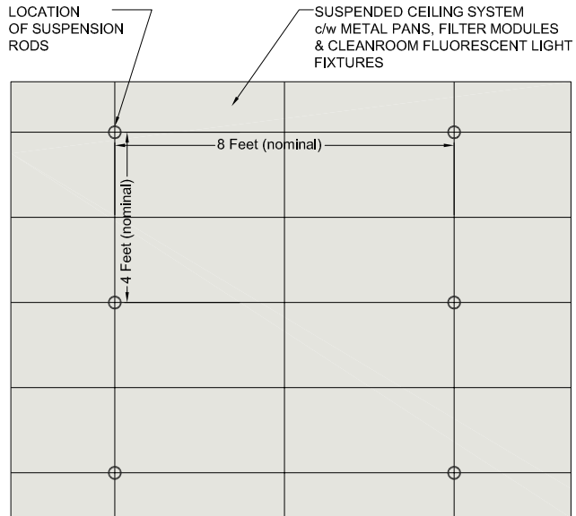
PARTIAL CEILING LAYOUT SHOWING LOCATION OF SUSPENSION RODS
