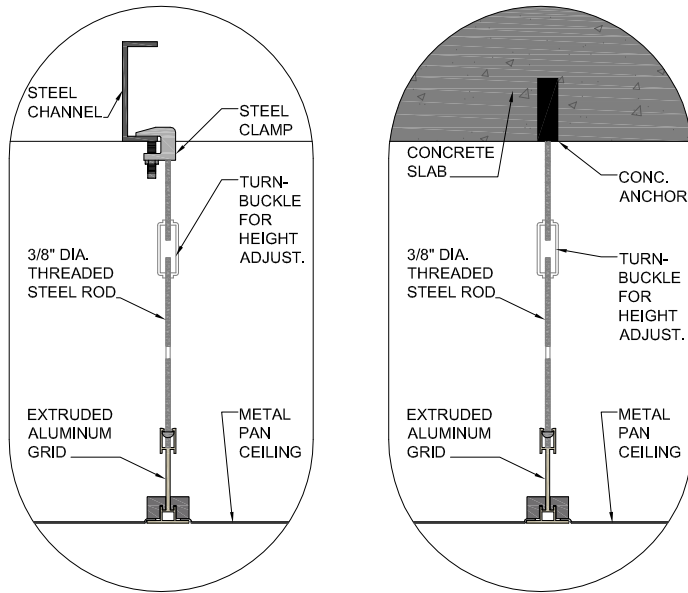
TYPICAL SUSPENSION DETAILS
