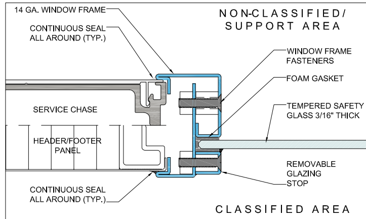
PARTIAL SECTION
