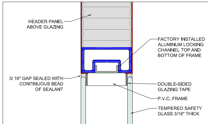
PARTIAL SECTION B-B
