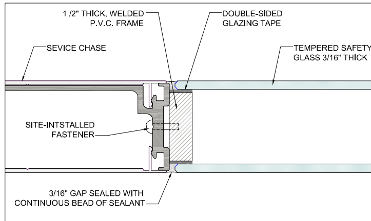
PARTIAL SECTION A-A
