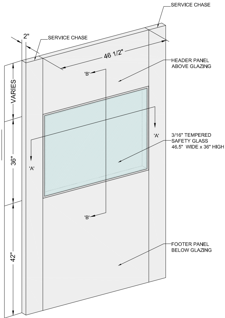
TYPICAL WINDOW ELEVATION
