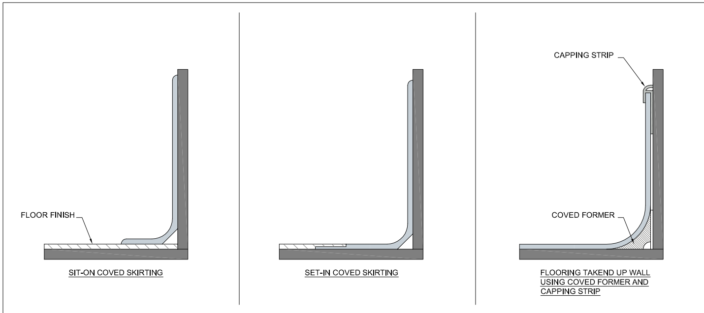
WALL/FLOOR INTERFACE DETAILS FOR PVC FLOORING
