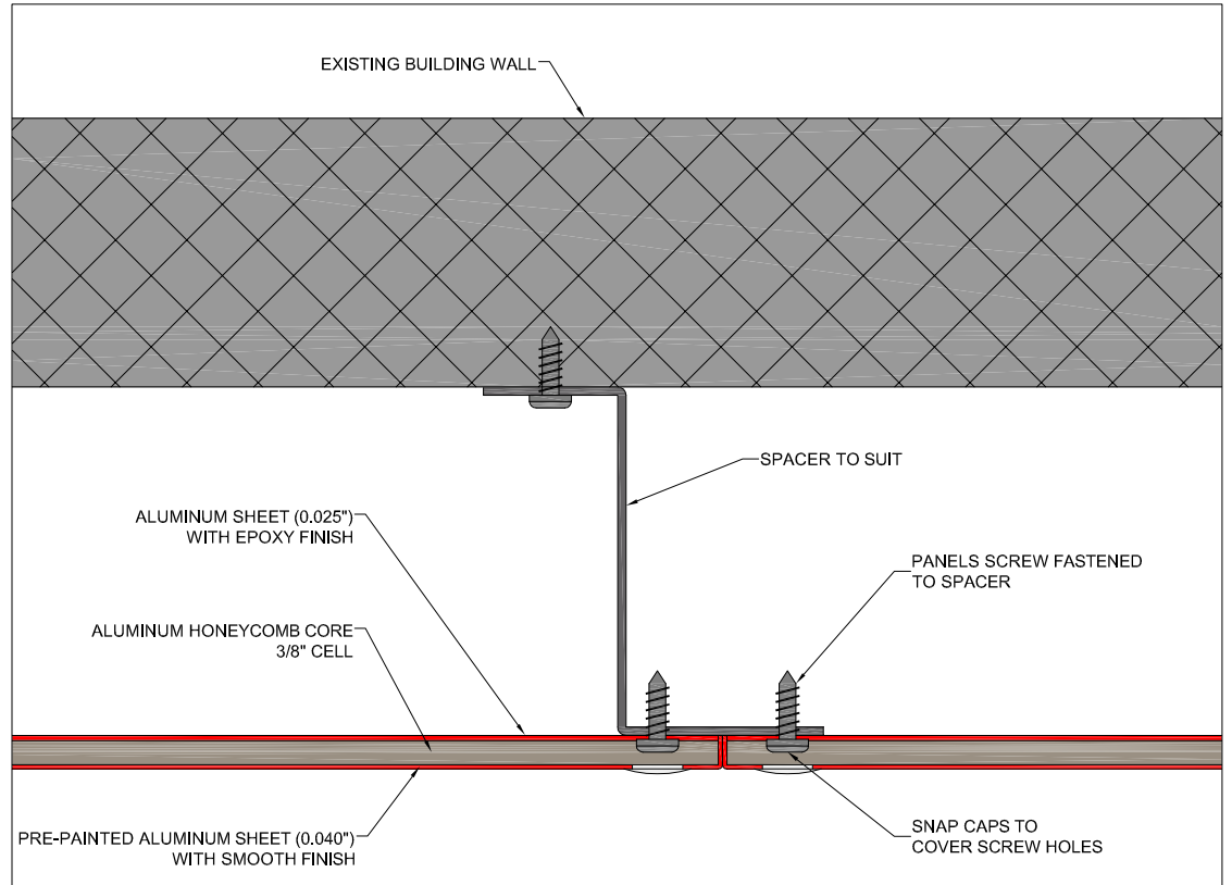
DETAIL A: ALTERNATIVE METHOD OF MOUNTING PRE-FINISHED 1/4" WALL PANELS TO EXISTING WALLS. SEE NOTE 1.
